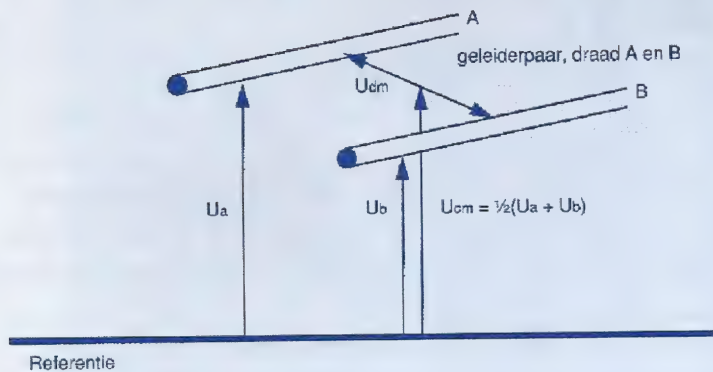
Figuur 1 Common mode (CM) en differential mode (DM) spanningen
